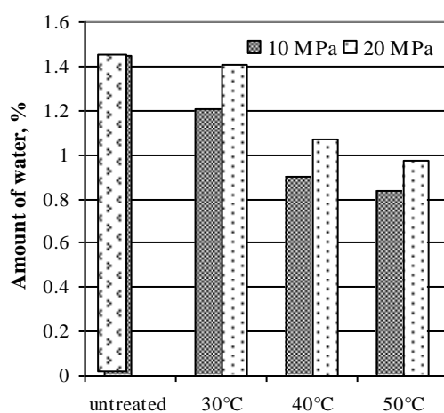
Figure 4. Water content in the lipase microenvironment after incubation (24 hours) in SC CO 2 at 10 MPa and 20 MPa and different temperatures
