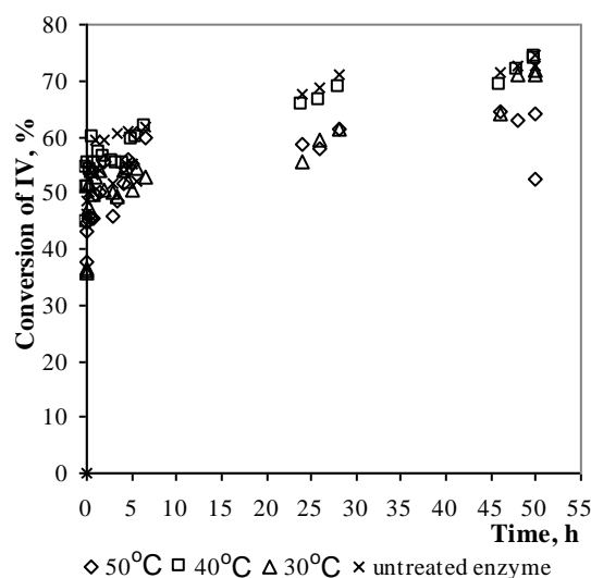
Figure 2. Conversion of IVs at 40°C and atmospheric pressure catalyzed by untreated lipase and lipase that was exposed to different temperatures in SC CO 2 at 10 MPa for 24 hours
