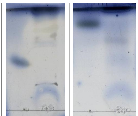
Figure 6. Acidic hydrolysis of tocopheryl glycoside. Start 1, on both plates, D,L- \alpha -tocopheryl- \beta -D-galactofuranoside; start 2, on both plates, hydrolysis product. Migration, plate one, SS IV, plate two – SS V. Visualisation, mostain.
