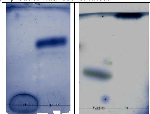
Figure 5. Peracetylation of tocopheryl glycoside. Start 1, on both plates, D,L- \alpha -tocopheryl- \beta -D-galactofuranoside; start 2, on both plates, peracetylated product. Migration, plate one, SS II, plate two – SS IV. Visualisation, mostain.
