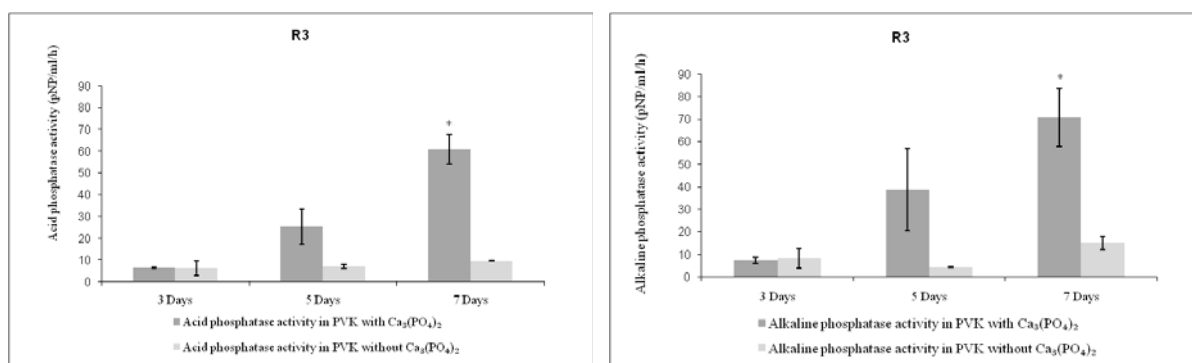
Figure 3. Acid and alkaline phosphatase activity in PVK broth with and without Ca 3 (PO 4 ) 2 . * - significant differences between sample and control.
