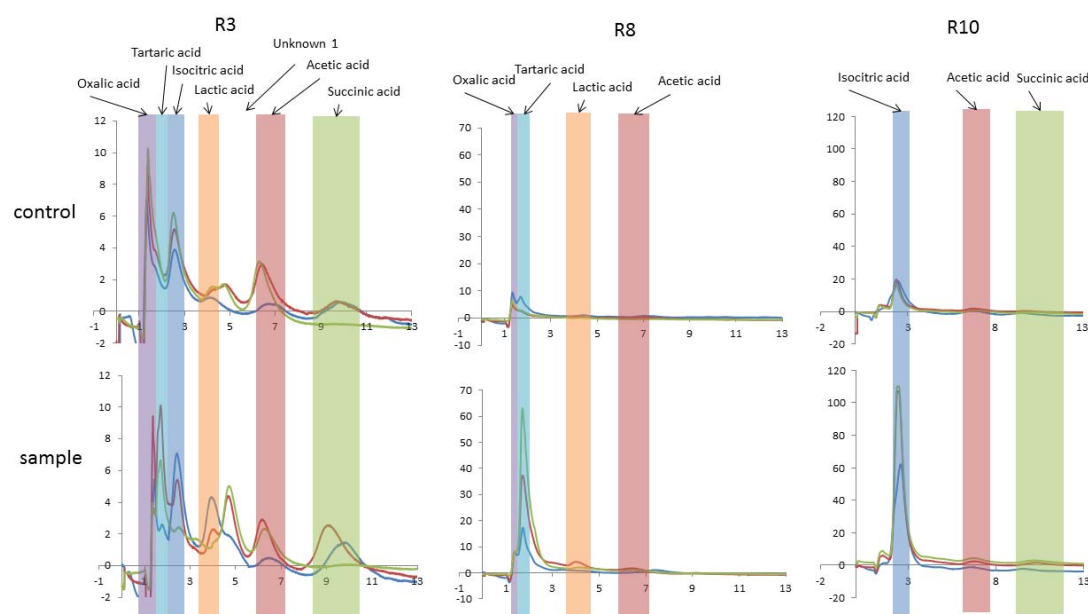
Figure 2. HPLC profiles of the culture filtrates for R3, R8 and R10 strains grown on PVK with (sample) and without \text{Ca}_3(\text{PO}_4)_2 (control) at various times: blue line - day 3, red line - day 5, green line - day 7.
