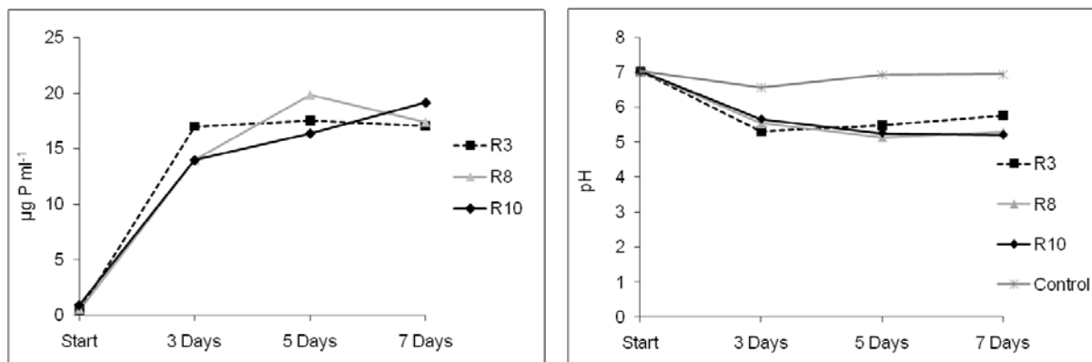
Figure 1. Changes in P-solubilization (left) and pH value (right) during 7 days of incubation in PVK broth.
